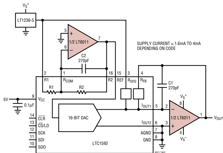
Low Power Programmable Output Range 16-Bit SoftSpan™ DAC
